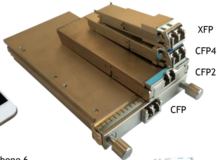
CFP4 vs. iPhone 6
